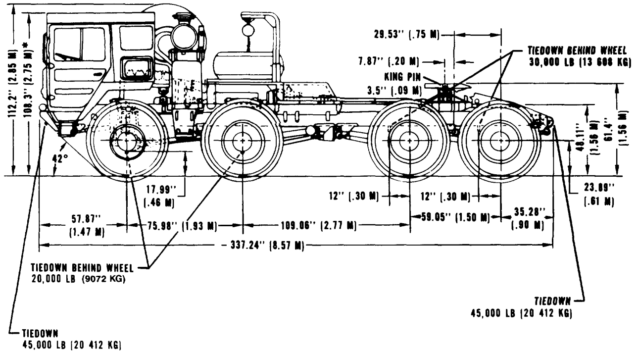
Figure 28. Left-side view of M1014 truck tractor.
