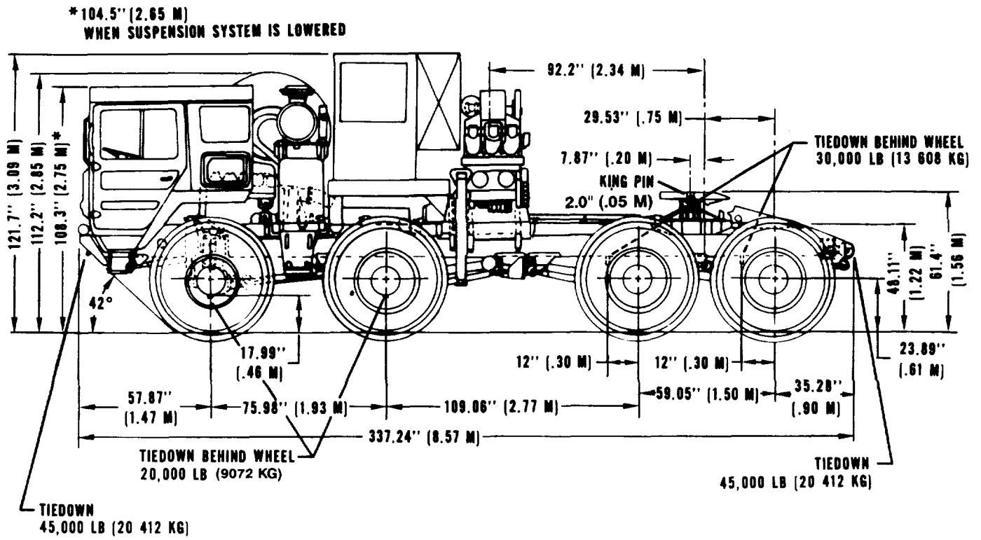
Figure 2-5. Left-side view of M1001 truck tractor.
