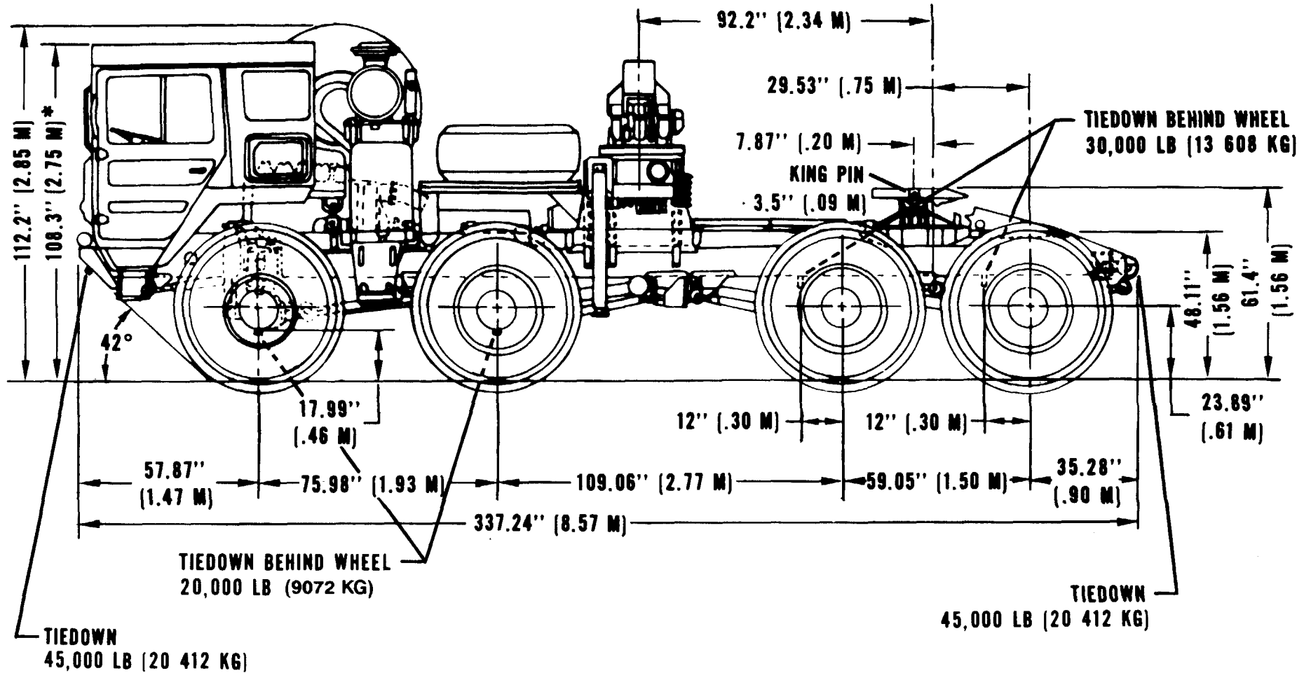
Figure 2-7. Left-side view of M1013 truck tractor.
